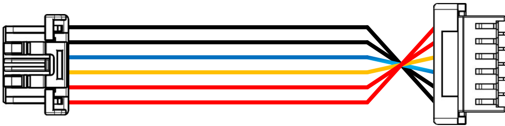
6-pin 2.0mm pitch to 6-pin 1.5mm pitch 200mm Cable x 1
